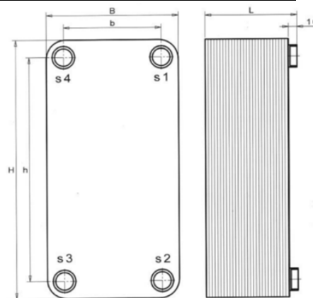
VM85 – G2"
