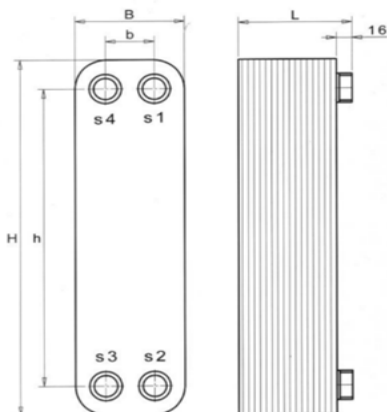
VM30 – G1"
